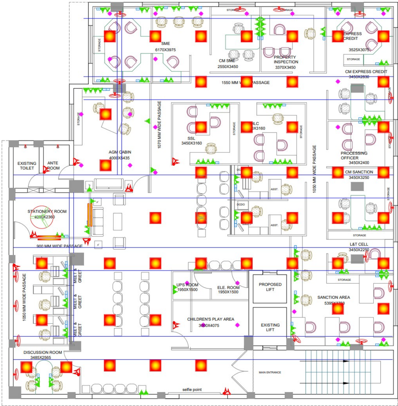
FIRST FLOOR SCHEMATIC PLAN
